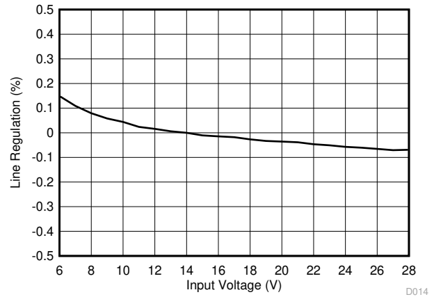
Figure 7-3. Line Regulation
