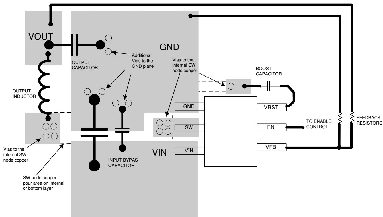
Figure 7-16. Board Layout
