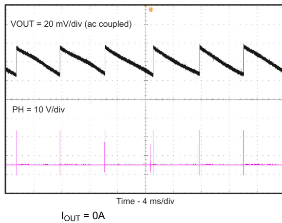
Figure 7-6. Output Voltage Ripple
