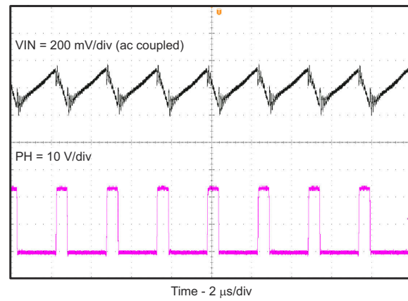
Figure 7-5. Input Voltage Ripple
