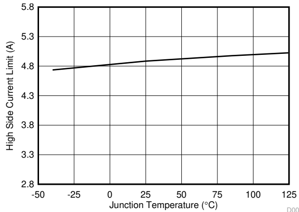
Figure 5-7. High-Side Current Limit Threshold vs Junction Temperature
