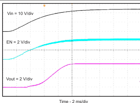
Figure 7-12. Start-Up Relative to VIN
