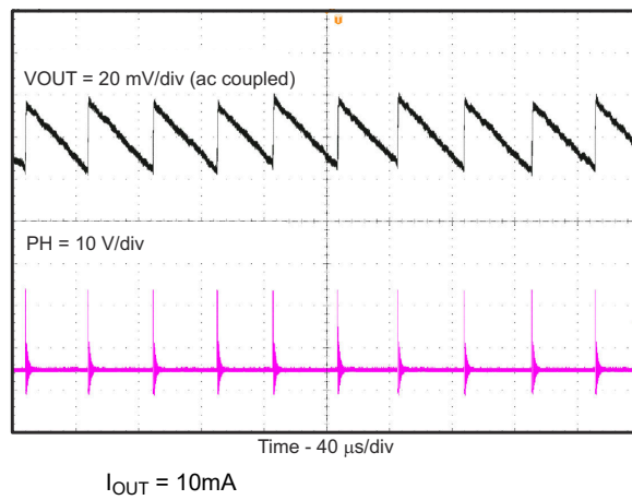
Figure 7-7. Output Voltage Ripple
