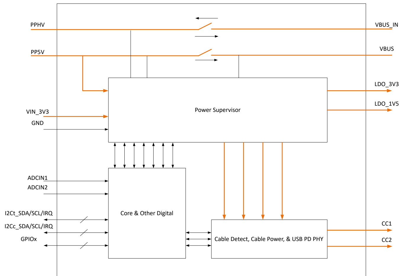
Figure 8-1. TPS25751D
