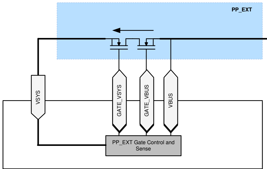
Figure 8-16. PP_EXT External Sink Path Control
