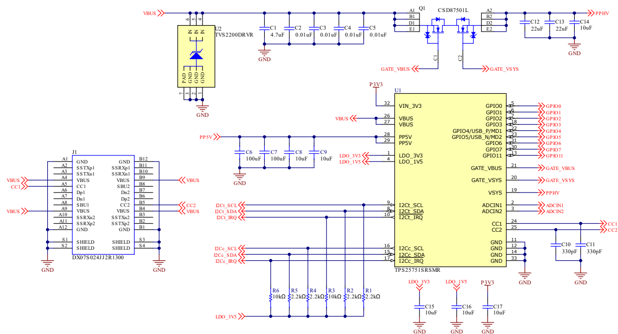
Figure 9-34. TPS25751S Example Schematic
