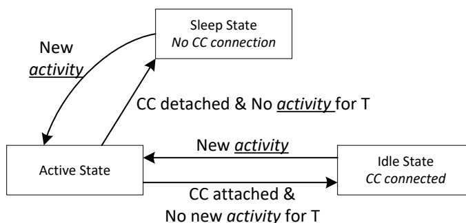
Figure 8-33. Flow Diagram for Power States
