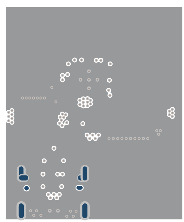
Figure 9-39. TPS25751S PCB Layout - GND Layer
