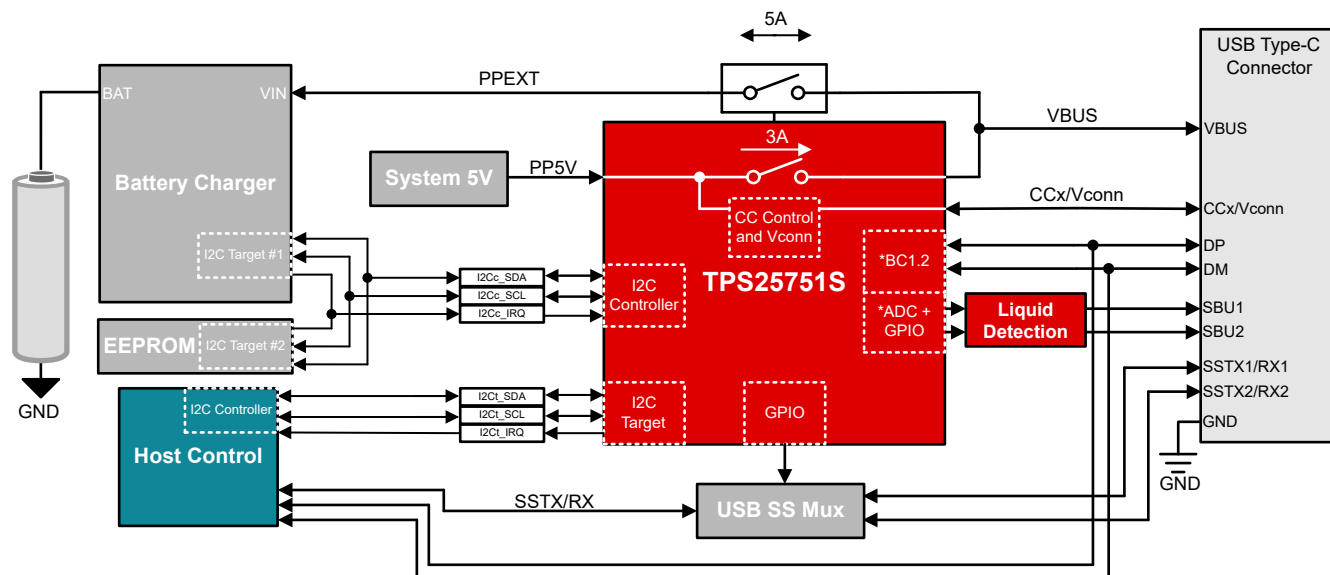
Figure 9-2. TPS25751S Battery Charger &amp; Full System Block Diagram
