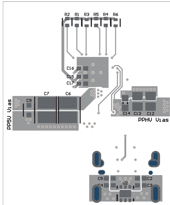
Figure 9-36. TPS25751S PCB Layout - Bottom Composite
