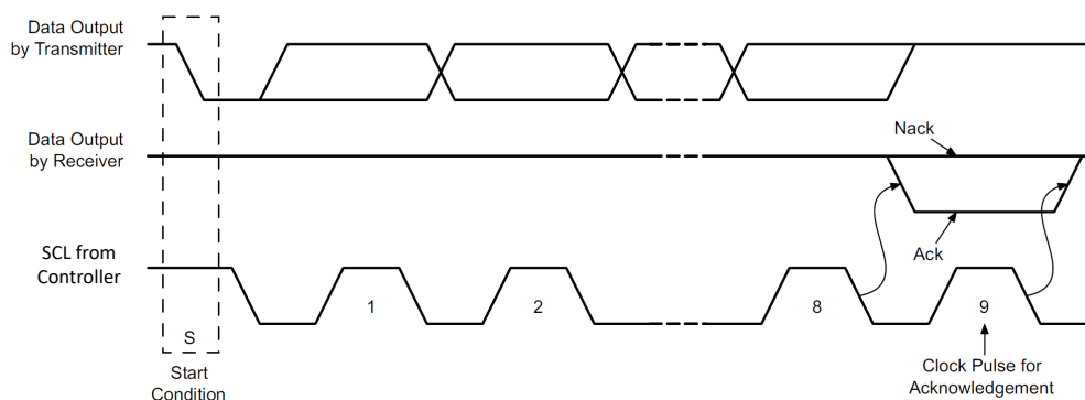
Figure 8-29. I²C Acknowledgment
