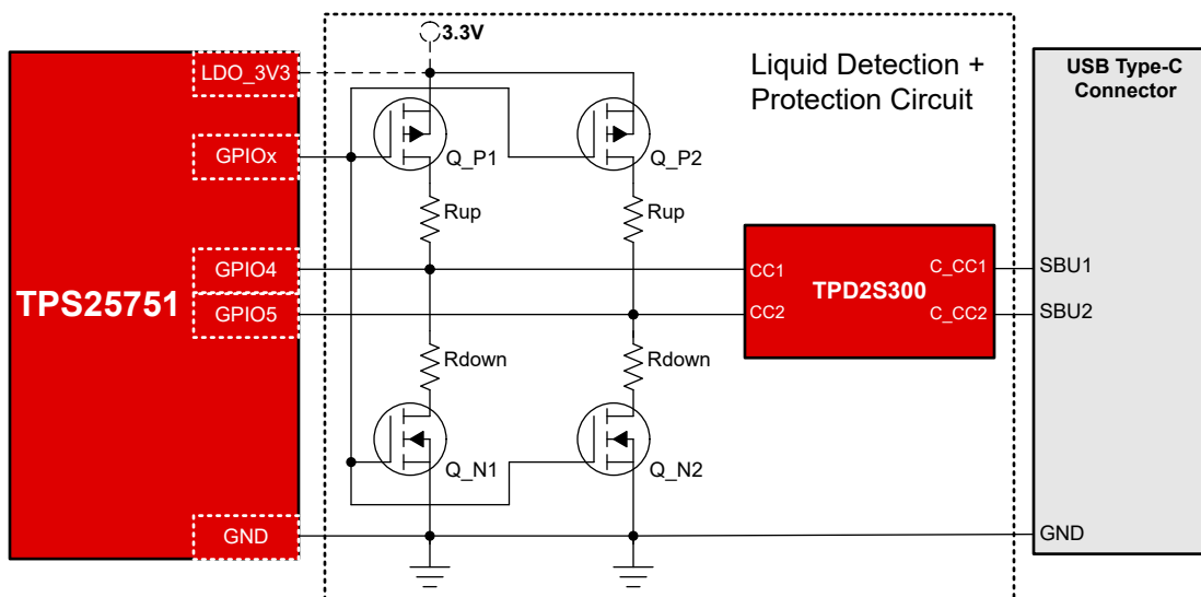
Figure 9-9. TPS25751 Liquid Detection Block Diagram - 1 GPIO Control
