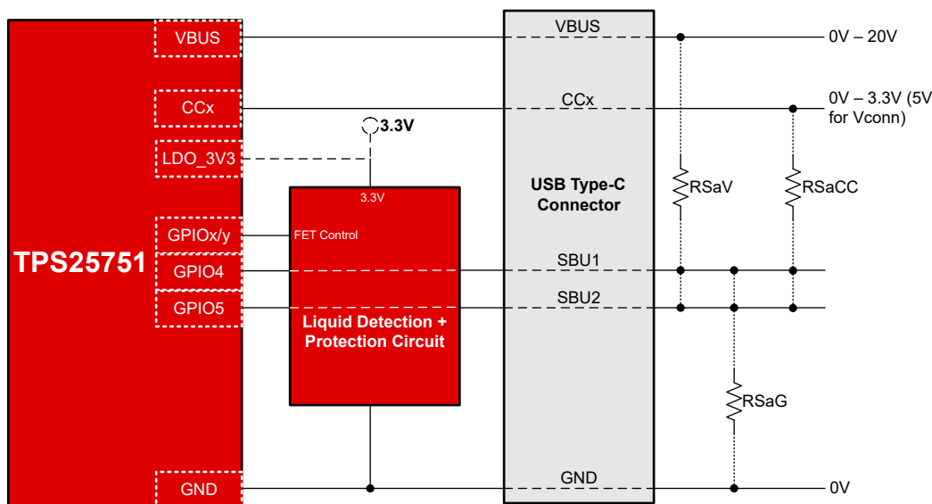
Figure 9-10. TPS25751 Liquid Detection Operation
