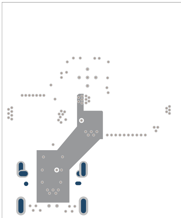
Figure 9-38. TPS25751S PCB Layout - Internal Power Layer
