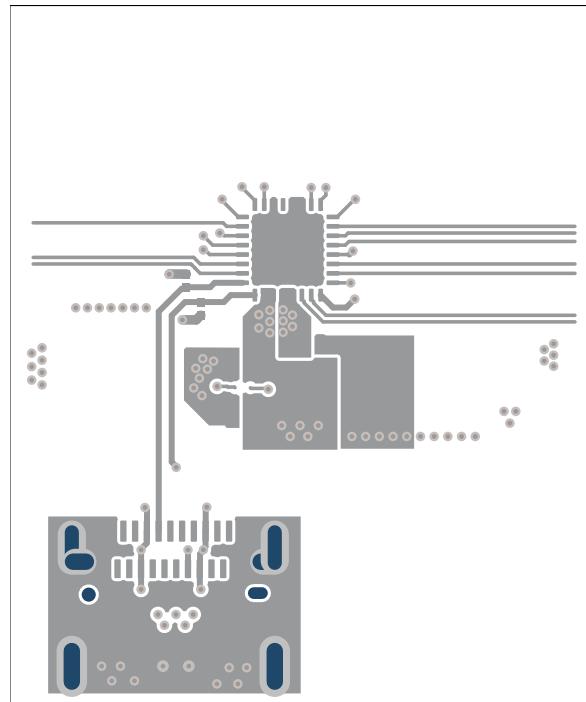
Figure 9-37. TPS25751S PCB Layout - Top Layer Routing
