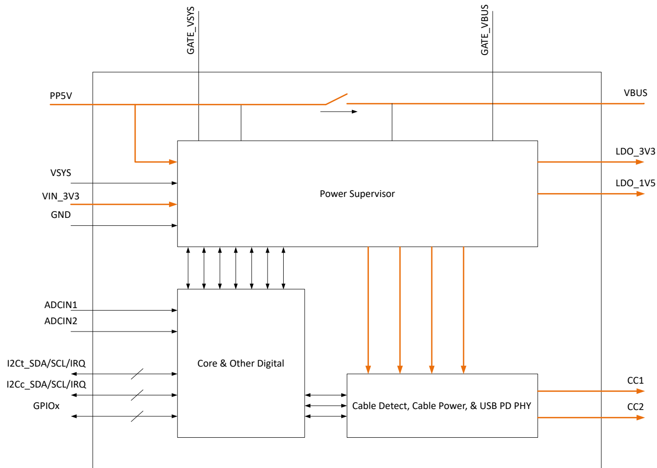
Figure 8-2. TPS25751S
