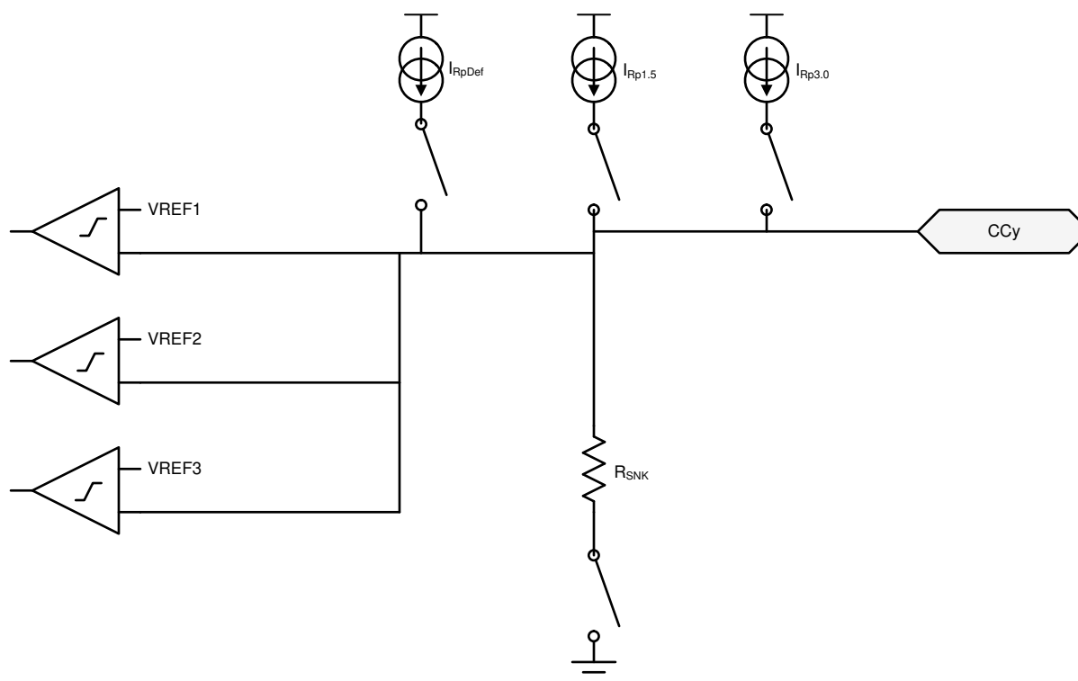
Figure 8-20. Plug and Orientation Detection Block
