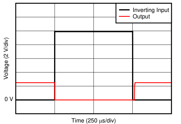
Figure 5-29. Inverting Differential Input Overload
