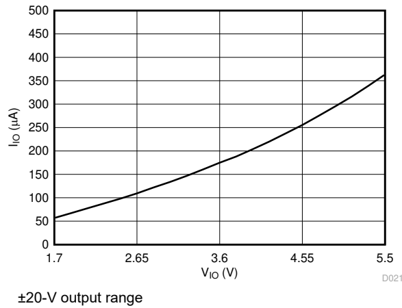
Figure 5-24. Supply Current ( I_{LO} ) vs Supply Voltage
