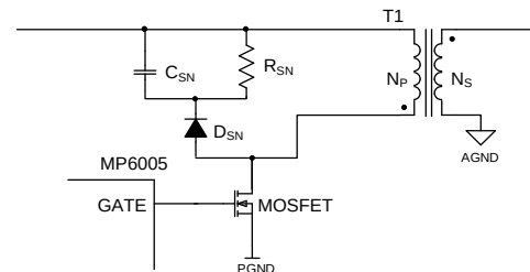
Figure 10: RCD Snubber
