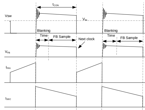
Figure 3: Continuous Conduction Mode (CCM) Condition Feedback Sample Control
