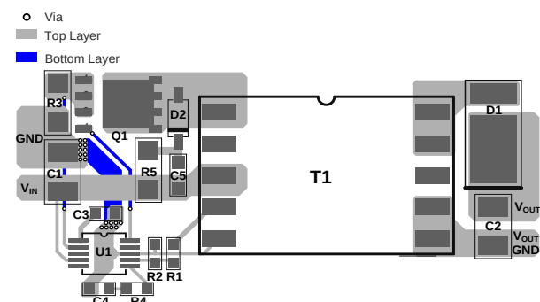
Figure 12: Recommended PCB Layout for Flyback Application (14)
