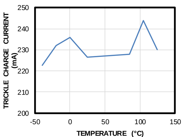
Trickle Charge Current vs. Temperature RS1 = 25m\Omega
