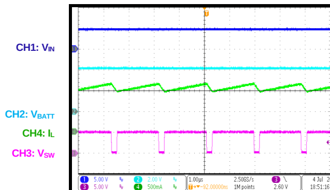
CV Charge Steady State
