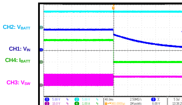
Shutdown, CC Charge Mode
