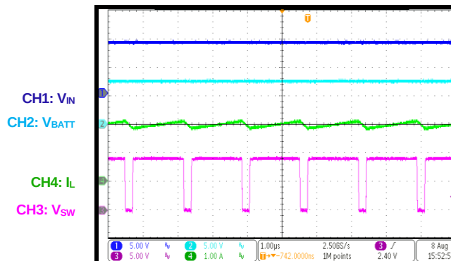
CC Charge Steady State (COT)
