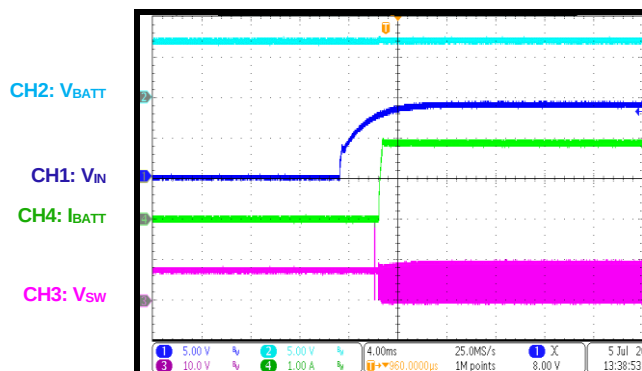
Start-Up, CC Charge Mode
