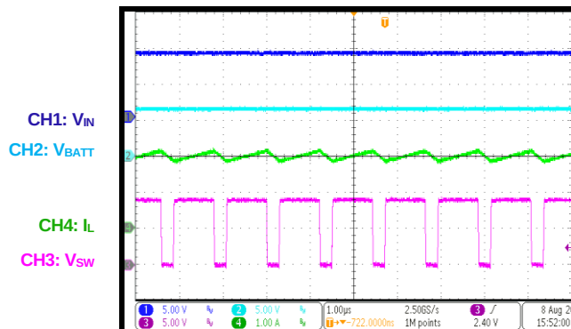
CC Charge Steady State
