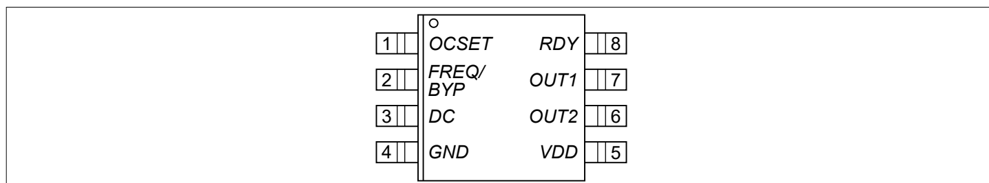
Figure 4 Pin-out for 2EP130R in PG-TSSOP-8 (top view)
