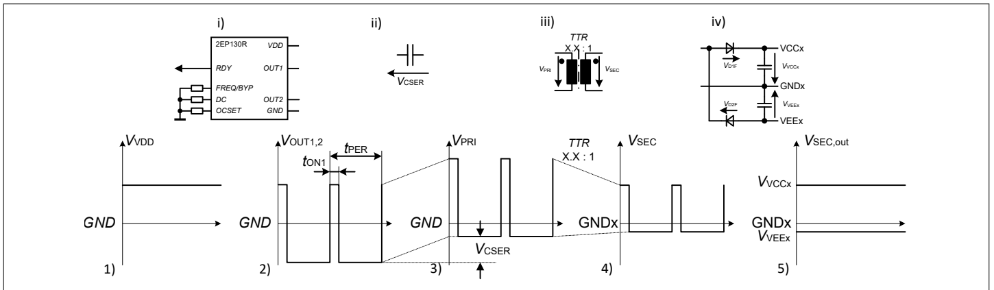
Figure 24 DC offset voltage and influence of transformer turns ratio output voltage
