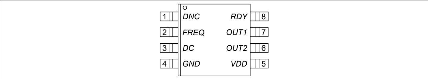
Figure 3 Pin-out for 2EP100R, 2EP101R, and 2EP110R in PG-TSSOP-8 (top view)
