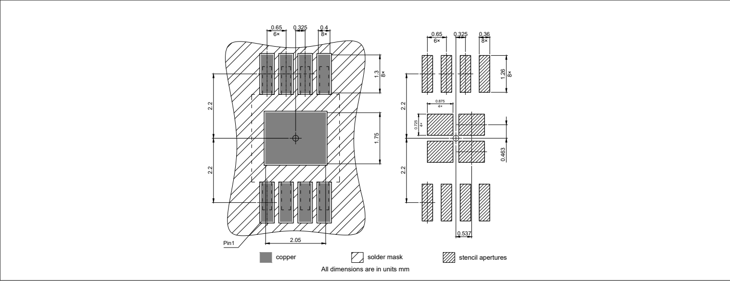
Figure 36 PG-TSSOP-8 footprint
