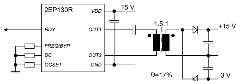
Schematic example for 2EP130R
